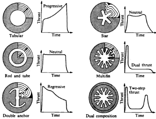
Gambar 2-1: Beberapa Grain Propelan Padat (Mattingly, 2006)
