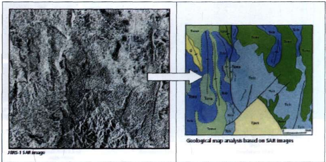
Fig. 11. Karst, which is unique in limestone areas, can be seen in this image taken by a microwave sensor (Synthetic Aperture Rader, SAR.) Although this area is vastly covered by a tropical rain forest and unevenness of the land surface can be observed (Sulawesi Island, Indonesia)
