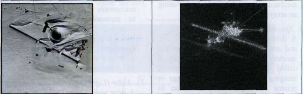
Fig. 5. This pair of images demonstrates some of the differences between passive and active sensors. The left image is an aerial photograph (which records reflected light) of Amundsen-Scott Station, a research facility built on the South Pole. The right image is the same area, at approximately the same scale and orientation, from RADARSAT
