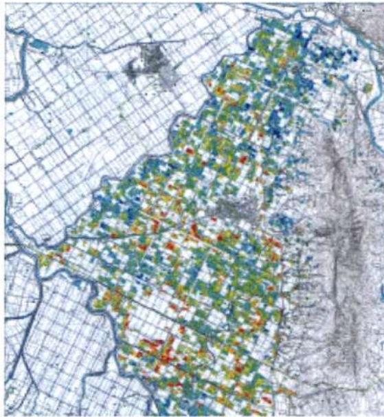
Fig. 8. Rice protein content map (SPOT/HRV Data, Sep. 5, 1999). Red and yellow areas indicate more protein in rice.
