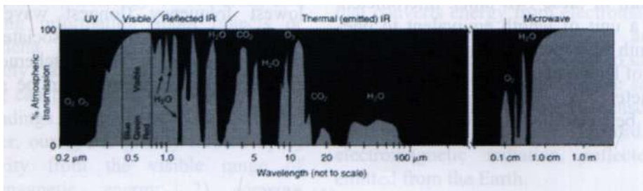
Fig. 2. Diagram of atmospheric windows—wavelengths at which electromagnetic radiation will penetrate the Earth's atmosphere. Chemical notation (CO 2 , O 3 ) indicates the gas responsible for blocking sunlight at a particular wavelength.
